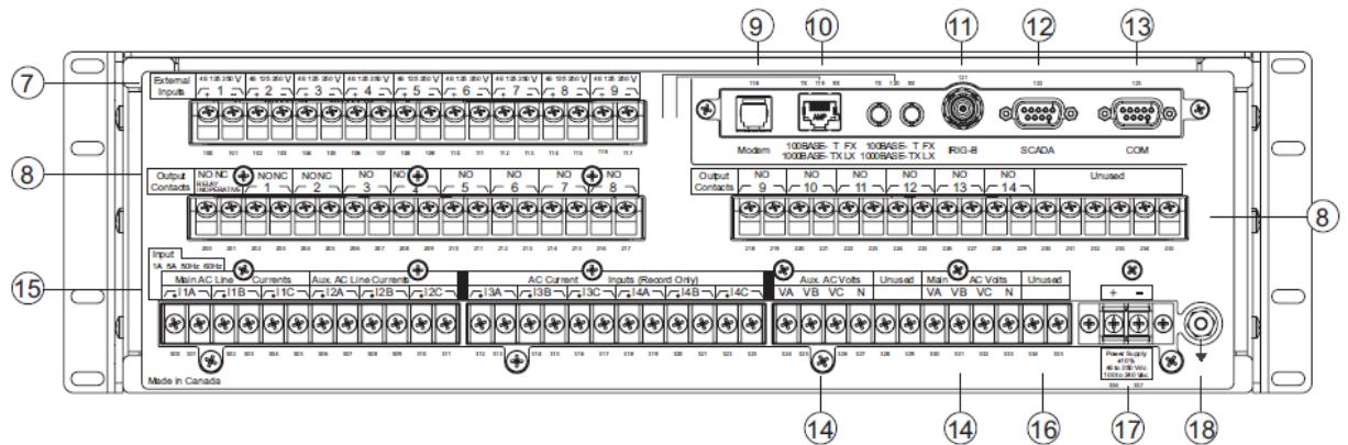
Figure 2 – L-PRO 4000 Relay Front View (4U)
