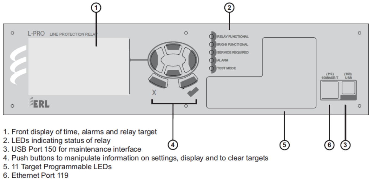
Figure 1 – L-PRO 4000 Front View (3U)
