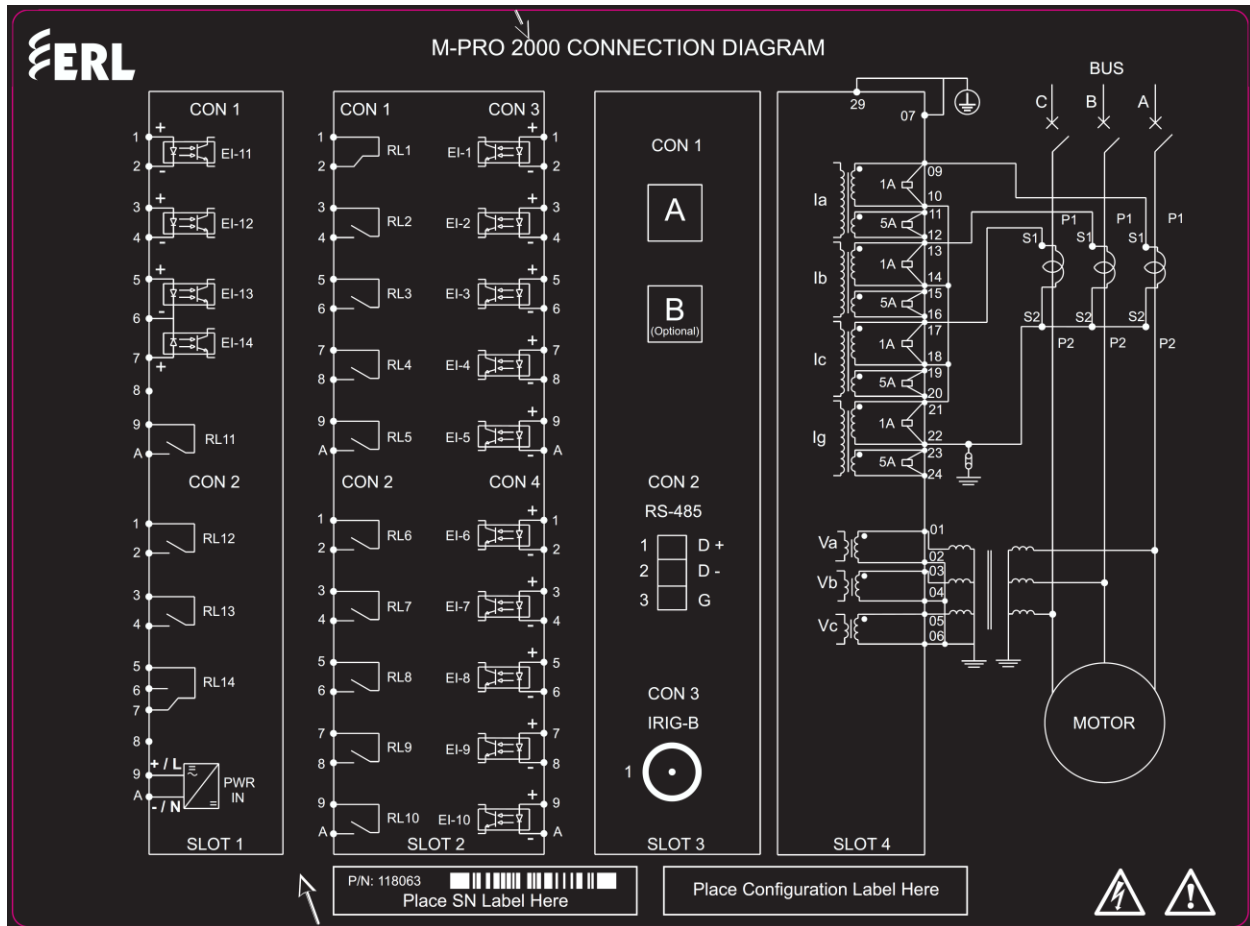
Figure 3 – Connection Diagram
