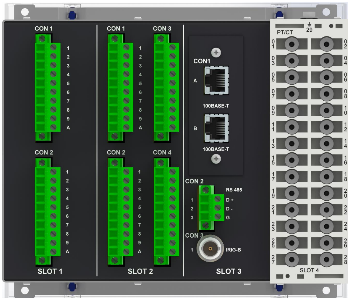
Figure 2 – M-PRO 2000 Relay Rear View
